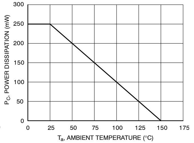
Figure 8. Power Derating
