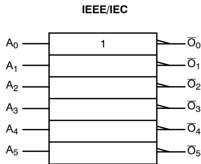
Figure 1. Logic Symbol
