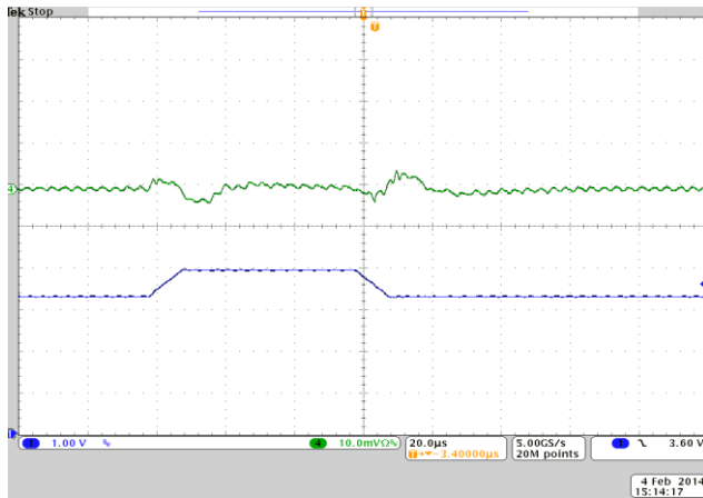
Figure 13. Line Transient, 5 mA Load, 10 \mu s Step
