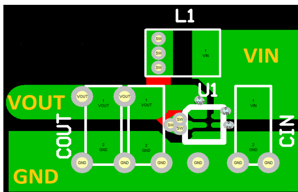
Figure 22. Layout Recommendation
