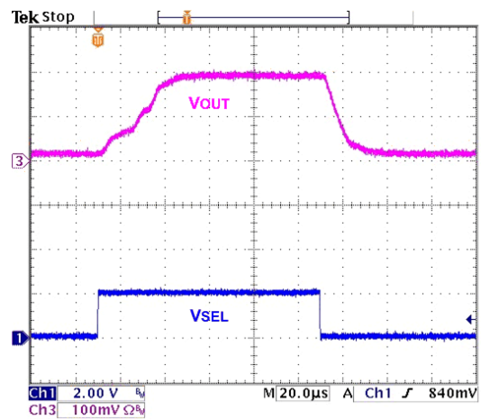
Figure 22. V_{SEL} Step, V_{IN} = 3.0\text{ V} , 500 mA Load
