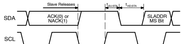
Figure 22. REPEATED START Timing
