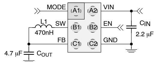
Figure 1. Typical Application
