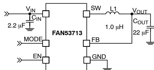
Figure 1. Typical Application
