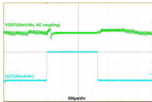
Figure 15. Load Transient, V_{IN} = 3.6\text{ V} , V_{OUT} = 1.8\text{ V} , 10 mA \leftrightarrow 150 mA, 1 \mu\text{s} Edge, Auto Mode
