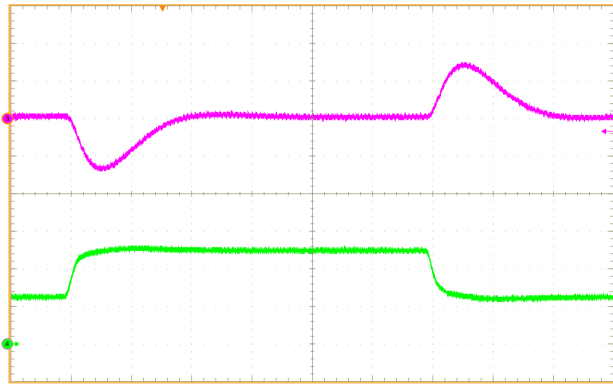
CH3 = V_o (0.4V/div), CH4 = I_{out} (2A/div), T = 50 \mu\text{s} /Div
