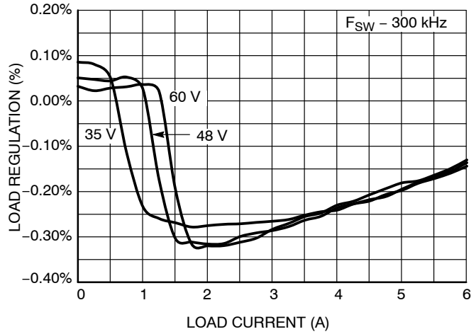
Figure 34. Load Regulation
