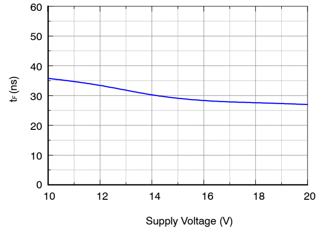
Figure 27. Turn-Off Fall Time vs. Supply Voltage
