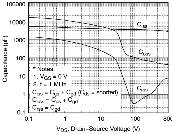
Figure 5. Capacitance Characteristics
