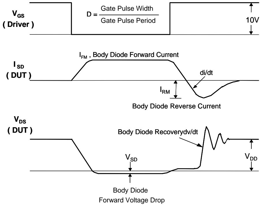
Figure 15. Peak Diode Recovery dv/dt Test Circuit & Waveform
