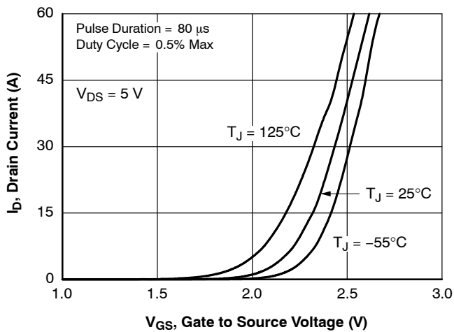
Figure 18. Transfer Characteristics
