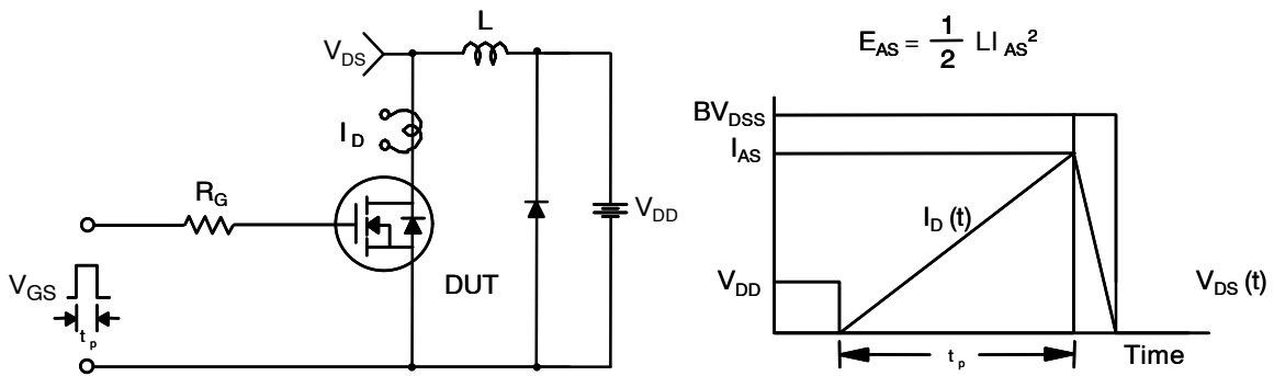
Figure 14. Resistive Switching Test Circuit & Waveforms
