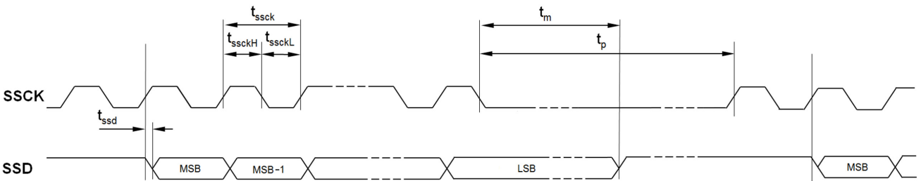
Figure 15: SSI Timing
