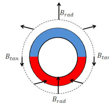
Figure 20: Side-Shaft Field
