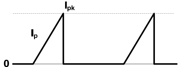
Figure 4: Primary Current Waveform
