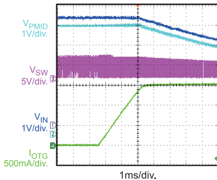
OTG Output CC Mode
