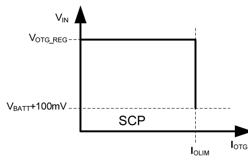
Figure 15: OTG Output U-I Curve
