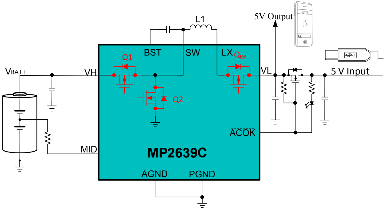
Figure 17: Two-Port Application
