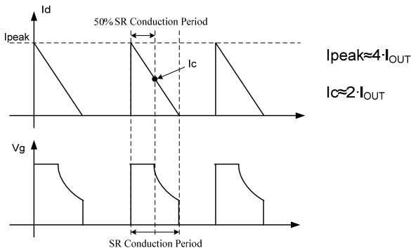
Figure 18: Synchronous Rectification Typical Waveforms in QR Flyback
