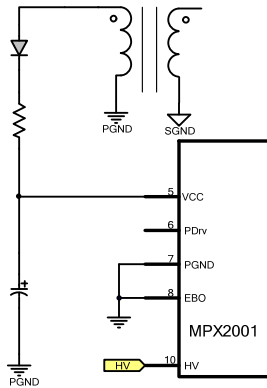
Figure 11: Start-Up Circuit
