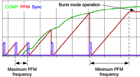
Figure 9: PFM Operation
