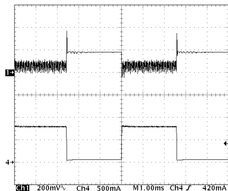
( V_{OUT} = 3.3\text{ V} , I_{LOAD} = 100\text{ mA to } 800\text{ mA} ; L = 5.6\ \mu\text{H} , C_{OUT} = 22\ \mu\text{F} ) Upper Trace: Output Voltage Ripple, 200 mV/Division Lower Trace: Load Current, I_{LOAD} , 500 mA/Division
