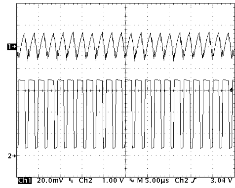
( V_{IN} = 2.5\text{ V} , V_{OUT} = 3.3\text{ V} , I_{LOAD} = 500\text{ mA} ; L = 5.6\ \mu\text{H} ) Upper Trace: Output Voltage Ripple, 20 mV/Division Lower Trace: Voltage at LX pin, 1.0 V/Division
