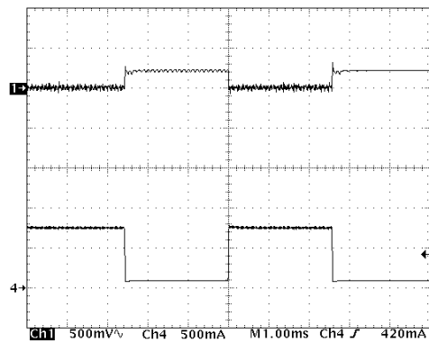
( V_{OUT} = 5.0\text{ V} , I_{LOAD} = 100\text{ mA to } 800\text{ mA} ; L = 5.6\ \mu\text{H} , C_{OUT} = 22\ \mu\text{F} ) Upper Trace: Output Voltage Ripple, 500 mV/Division Lower Trace: Load Current, I_{LOAD} , 500 mA/Division
