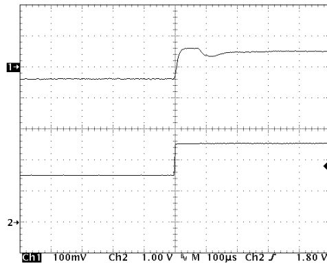
( V_{IN} = 1.5\text{ V to } 2.5\text{ V} ; L = 5.6\ \mu\text{H} , C_{OUT} = 22\ \mu\text{F} , I_{LOAD} = 100\text{ mA} ) Upper Trace: Output Voltage Ripple, 100 mV/Division Lower Trace: Battery Voltage, V_{IN} , 1.0 V/Division
