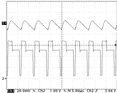
( V_{IN} = 2.5\text{ V} , V_{OUT} = 3.3\text{ V} , I_{LOAD} = 50\text{ mA} ; L = 5.6\ \mu\text{H} ) Upper Trace: Output Voltage Ripple, 20 mV/Division Lower Trace: Voltage at Lx pin, 1.0 V/Division
