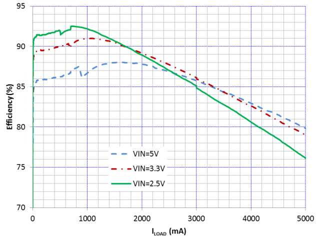
Figure 15. Efficiency vs I_{LOAD} and Temperature, V_{OUT} = 1.394 V
