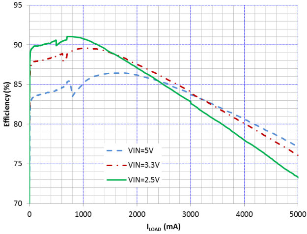
Figure 10. Efficiency vs I_{LOAD} and V_{IN} , V_{OUT} = 1.150 V
