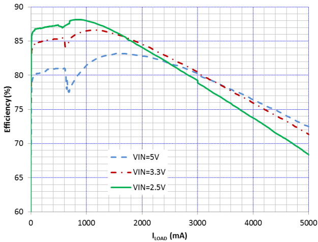
Figure 14. Efficiency vs I_{LOAD} and Temperature, V_{OUT} = 0.906 V , HEI201612A-R24M Inductor
