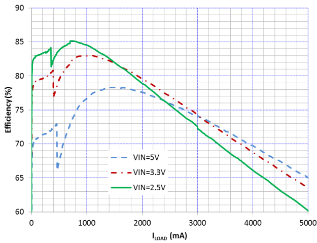
Figure 12. Efficiency vs I_{LOAD} and V_{IN} , V_{OUT} = 0.600 V
