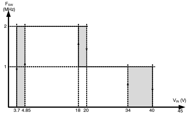
Figure 43. High Voltage Frequency Foldback
