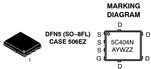
N-CHANNEL MOSFET
