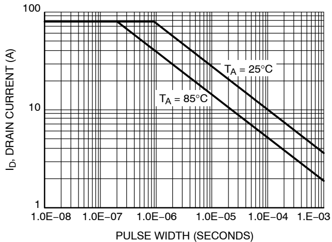
Figure 16. Avalanche Characteristics
