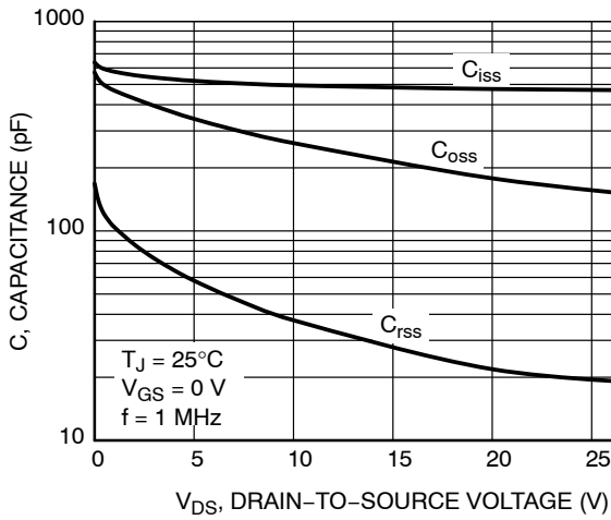
Figure 7. Capacitance Variation
