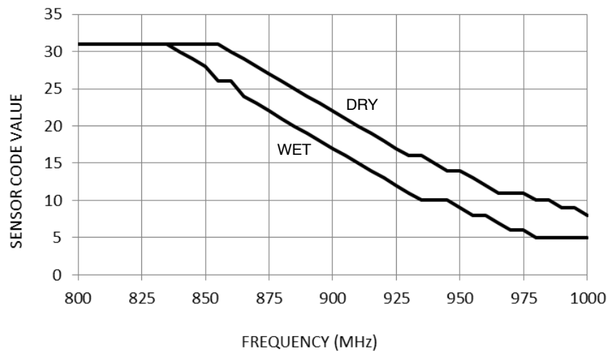
Figure 2. Sensor Code for Wet and Dry Conditions
